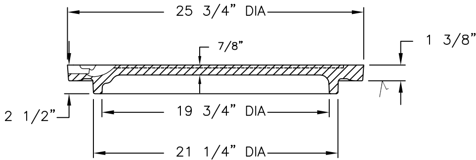
COVER SECTION
