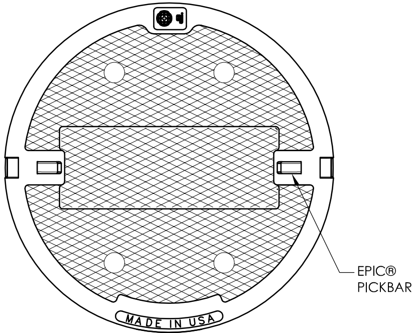
PLAN VIEW
