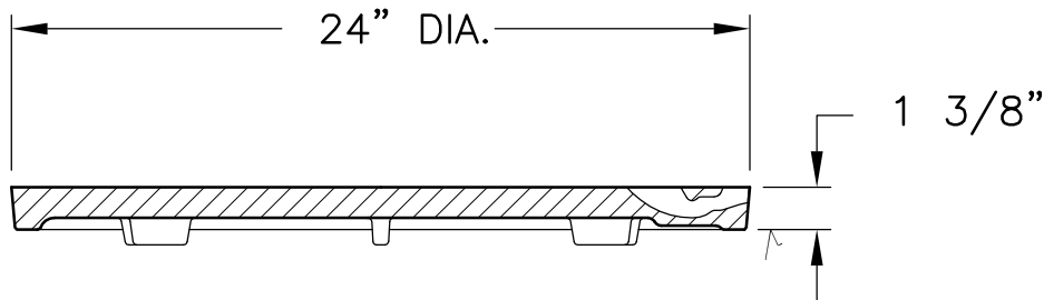
SECTION VIEW
