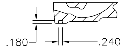
PICKHOLE DETAIL & GASKET GROOVE DETAIL
