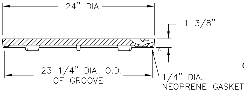
SECTION VIEW
