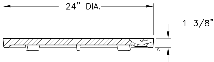
SECTION VIEW
