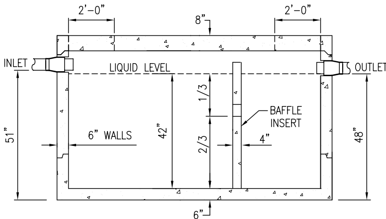
REVISED 2500 - 5000 HD Septic Tank drawings
