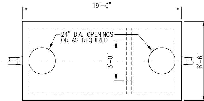
REVISED 2500 - 5000 HD Septic Tank drawings
