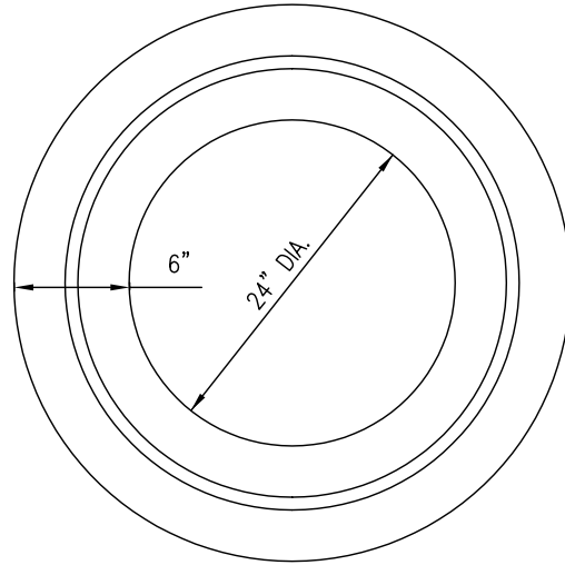
Plan (Jointed)
